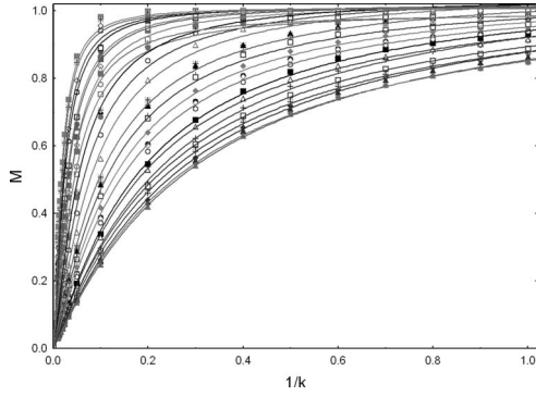
FIG. 4. Illustration of the power-law dependence of the information mobility on the fractional time for 38 real-world networks. It is seen that as the time progresses from 0 to 1 the information mobility grows following a power-law. At infinite times, a value of M=1 is obtained.
