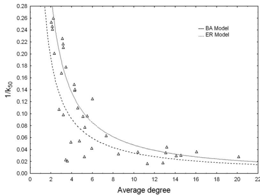
FIG. 5. Illustration of the relation between the half-time parameter and the average degree for 38 real-world networks. The plots obtained for the random networks are given for analyzing the performance of the real-world networks with respect to the random ones.
