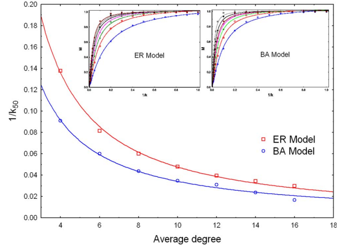
FIG. 3. (Color online) (Inner panels) Illustration of the power-law dependence between the information mobility and the fractional time for random networks with Poisson and scale-free degree distributions. It is seen that as the time progresses the mobility grows until reaching a saturation at values about 1/k=1 . (Main panel) Relation between the information mobility half time and the average degree for the random networks generated by ER and BA models. It is observed that as the average degree increases the mobility half time goes to zero following a power-law decay. For small average degree it is seen that scale-free networks (BA) display a larger mobility half time than ER networks.
