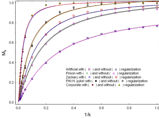
FIG. 2. (Color online) Illustration of the results obtained by calculating the fractional powers of the transition matrix with and without regularization for the artificial network illustrated in Fig. 1 and for four real-world networks.
