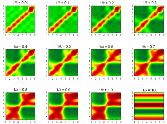
FIG. 1. (Color online) (a) An artificial network used to illustrate the process of information mobility (b) for different values of fractional times 1/k < 1 . The transition matrix for the value 1/k=100 is also illustrated as a representation of the stationary state.
